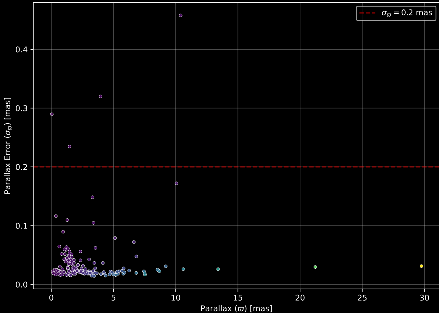
APOGEE DR17 Field: [K2_C8_122-57_btx] Parallax Quality (n= 181)
