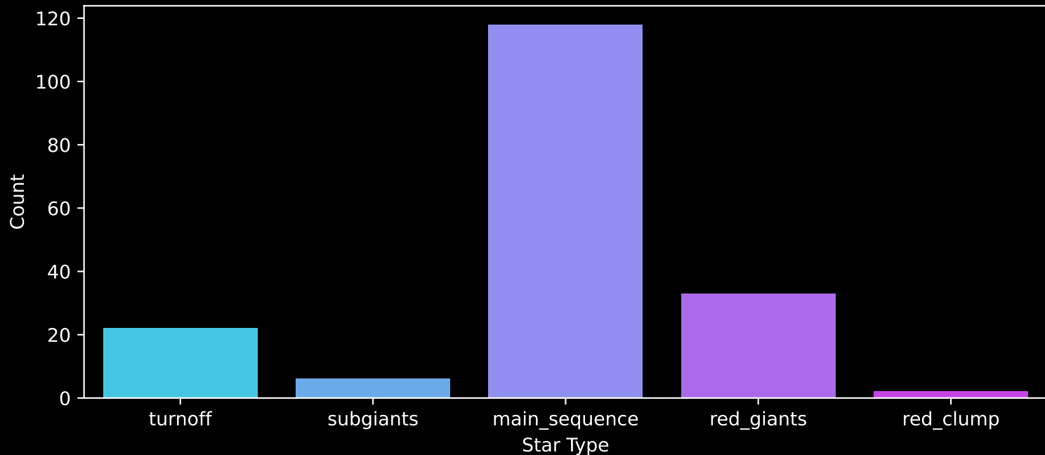
APOGEE DR17 Field: [K2_C8_122-57_btx] Count plot of Star Type
