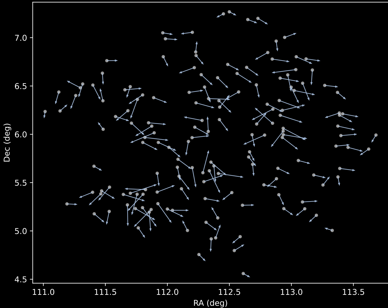
APOGEE DR17 Cluster 1 Proper Motion Vectors (n=157)
