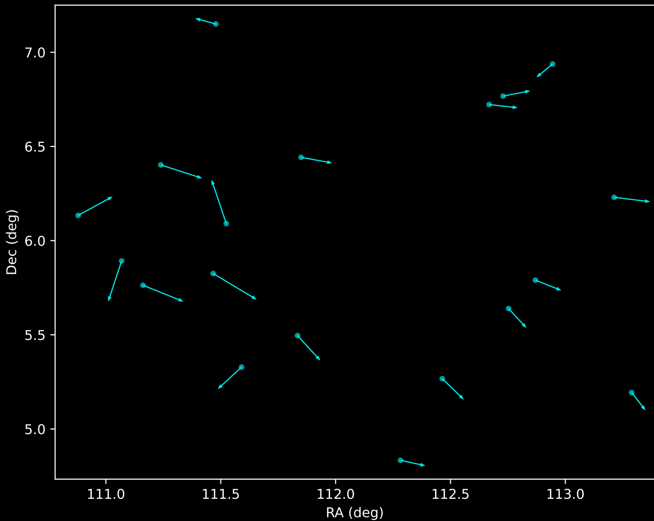
APOGEE DR17 Noise Stream Proper Motion Vectors (n=19)
