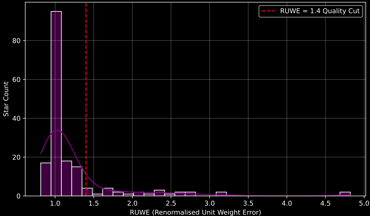
GAPOGEE DR17 Field [K2_C8_122-57_btx] RUWE Distribution (n= 172)
