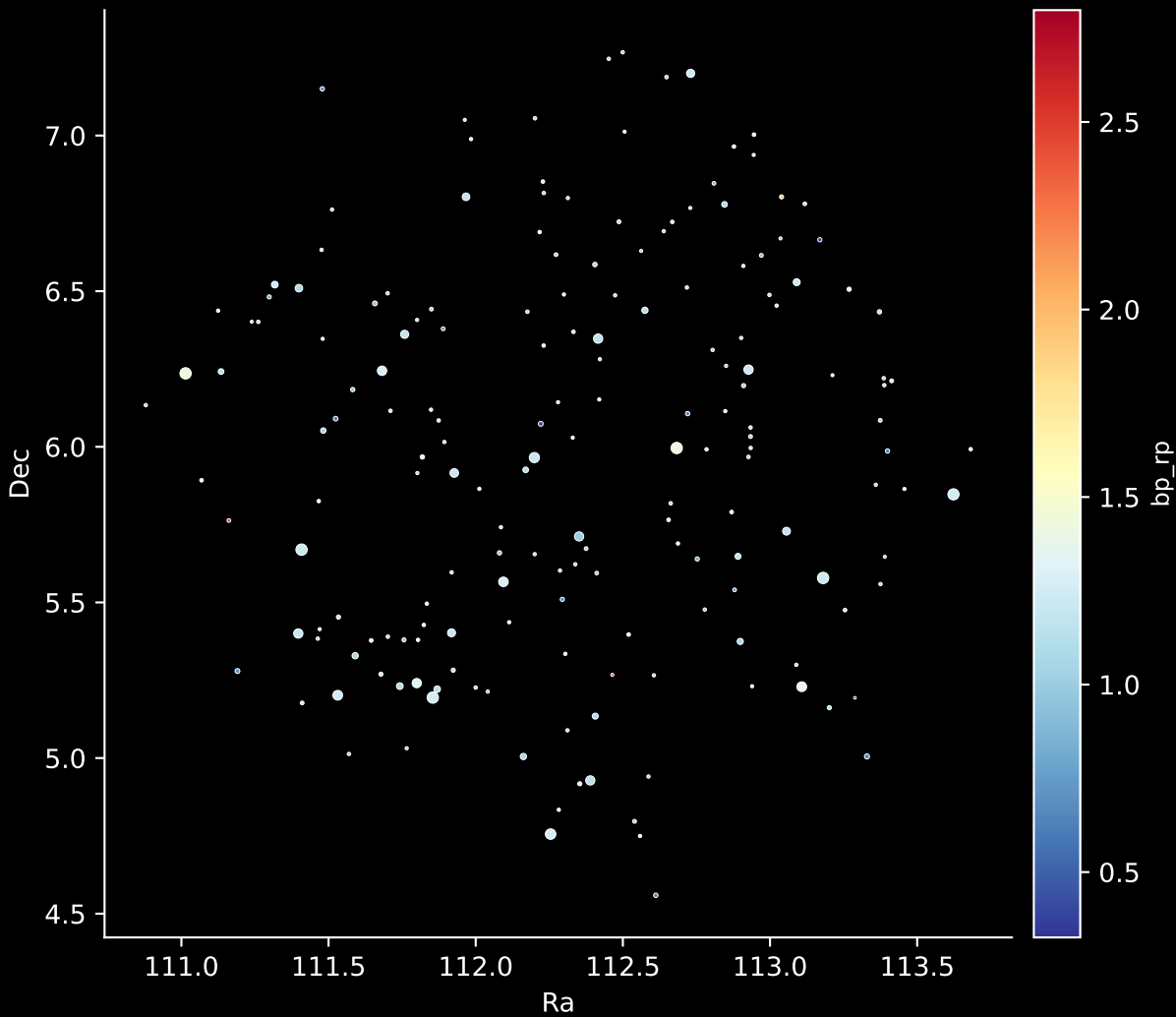
APOGEE DR17 Field: [K2_C8_122-57_btx] Stars: 181
