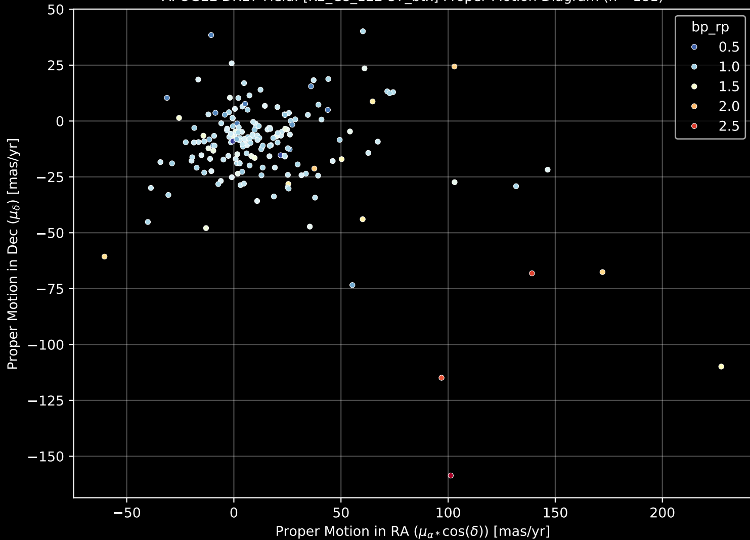
APOGEE DR17 Field: [K2_C8_122-57_btx] Proper Motion Diagram (n= 181)
