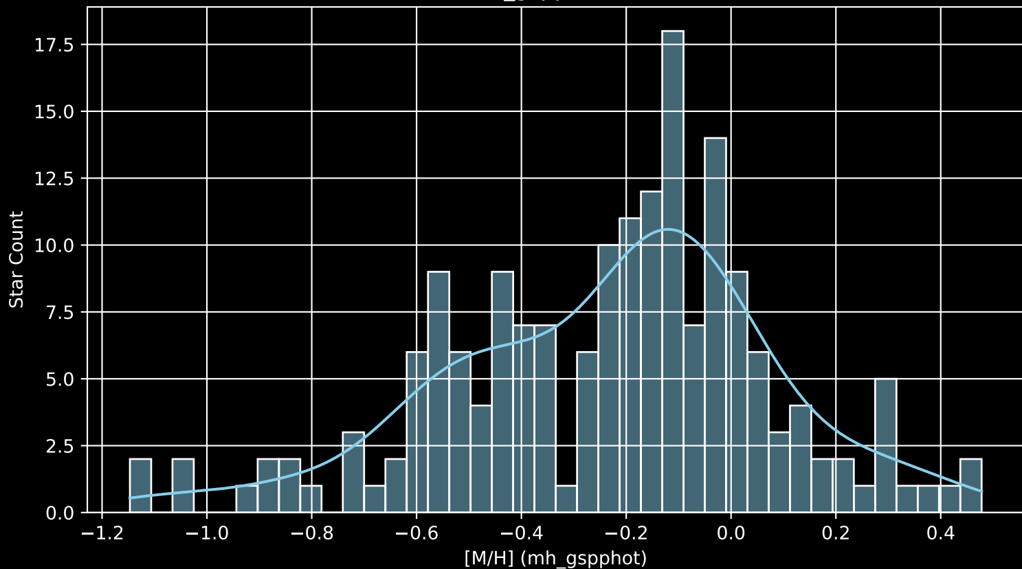
APOGEE DR17 Field: [K2_C8_122-57_btx [M/H] (mh_gspphot) (n= 180)
